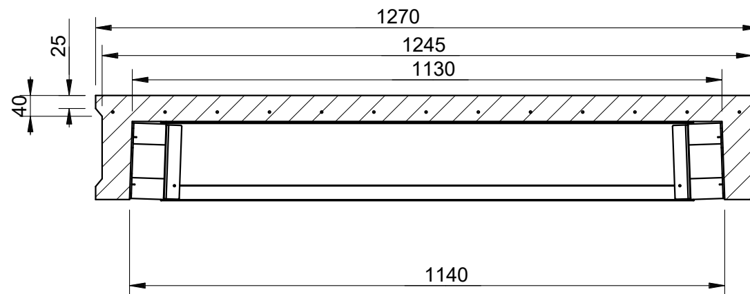
Section B-B
